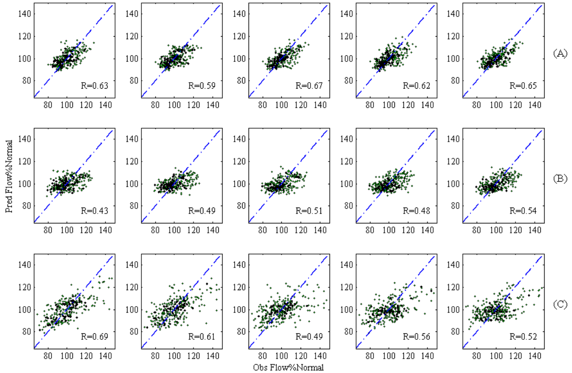
Figure 11: Scatter plots between measured and predicted streamflow for M5P using a 10-year moving average for (A) Colorado River near Cisco, Utah; (B) Green River at Green River, Utah; and (C) San Juan River near Bluff, Utah. The diagonal line is the 45° bisector line. Plots are shown with a 1-year lag on the left and ascending to a 5-year lag on the right.
