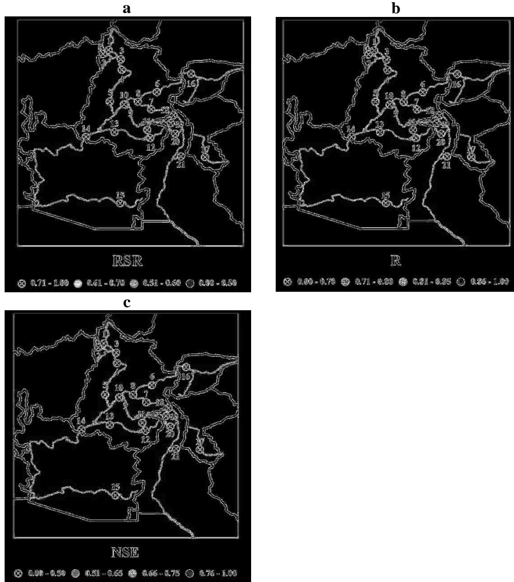
Figure 46: MLR results at a 1-year lead-time displayed in a spatial map for (a) RSR, (b) R, and (c) NSE.
